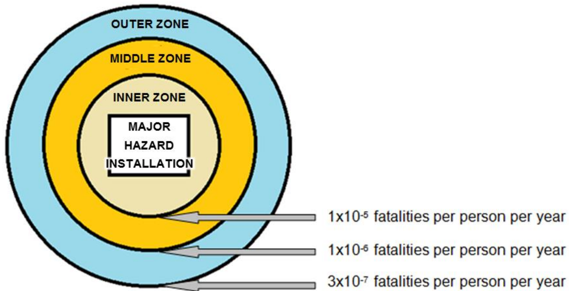
Figure 4.5: Town-planning zones
